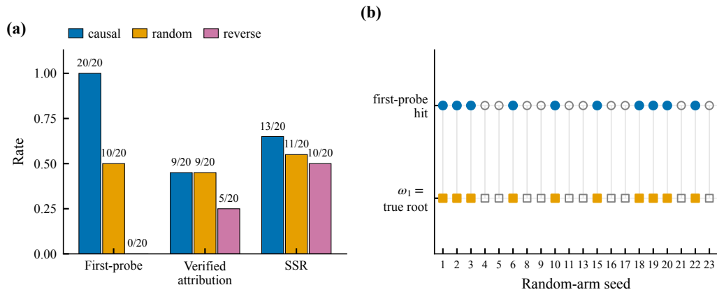
Figure 3: Exp-A commitment-order ablation and alignment audit (measured; snapshot mode; n=20/\text{order} ; plant me_force_zero_sea). (a) First-probe hit, verified attribution, and SSR@K by probe order. (b) Seed-level alignment audit of the random arm: a first-probe hit occurs if and only if the committed shuffle places the guilty layer first ( \omega_1 = a^* ; 10/10 with zero exceptions) — the random arm’s naming performance is carried entirely by accidental alignment with the ranking. Seeds 7, 12, 14 had no completed run manifest and are outside the campaign’s n=20 .
