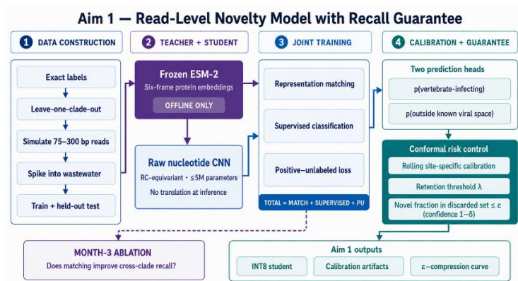
Figure 1. Aim 1 workflow for distilling a compact read-level novelty model from a frozen ESM-2 teacher through representation matching, supervised learning, and positive–unlabeled learning.
