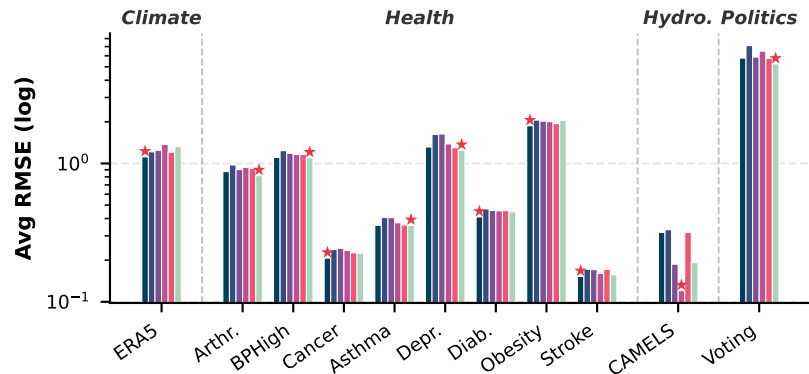
Avg RMSE
