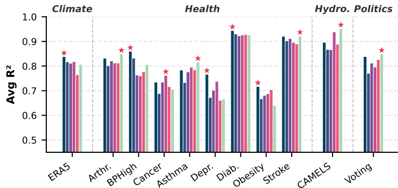
Avg R 2
