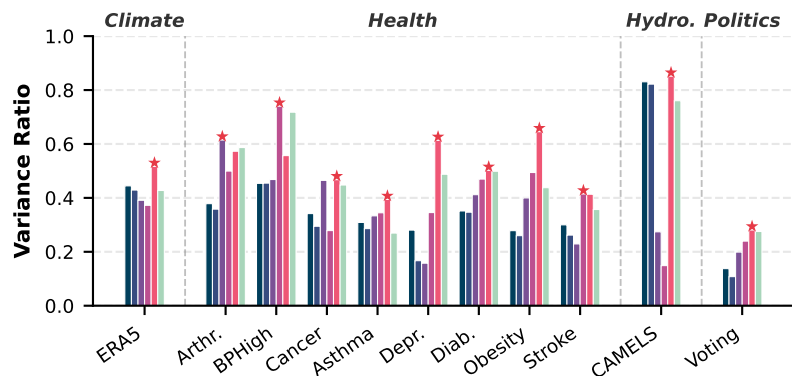
Variance Ratio
