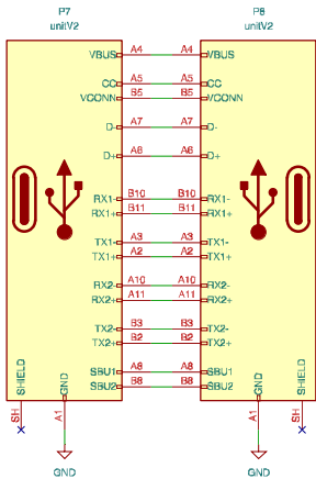
Connector_unitV2
