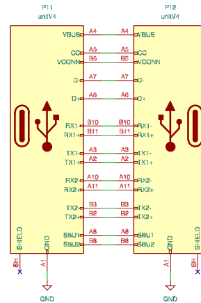
Connector_unitV4
