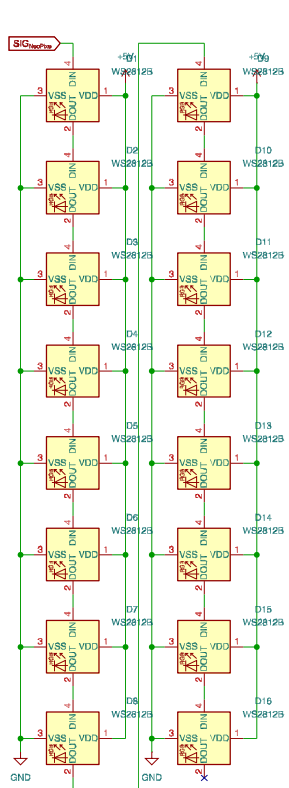
NeoPixel
