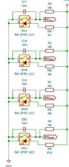
Switch
