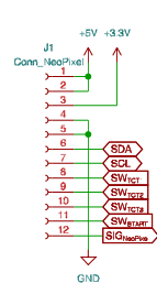
Connector_Sub
