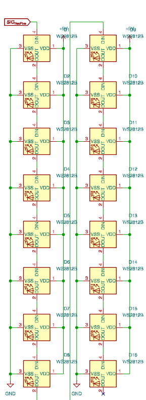
NeoPixel
