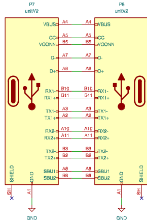
Connector_unitV2
