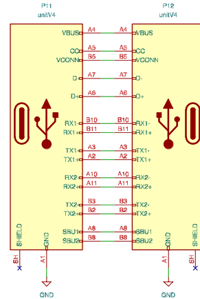
Connector_unitV4
