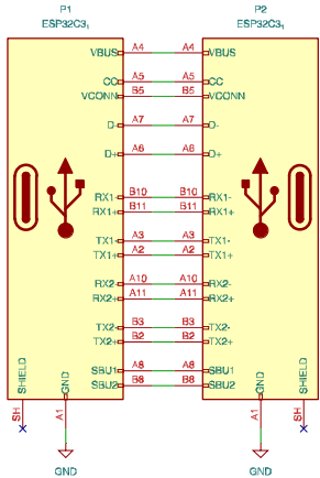
Connector_ESP32C3 1
