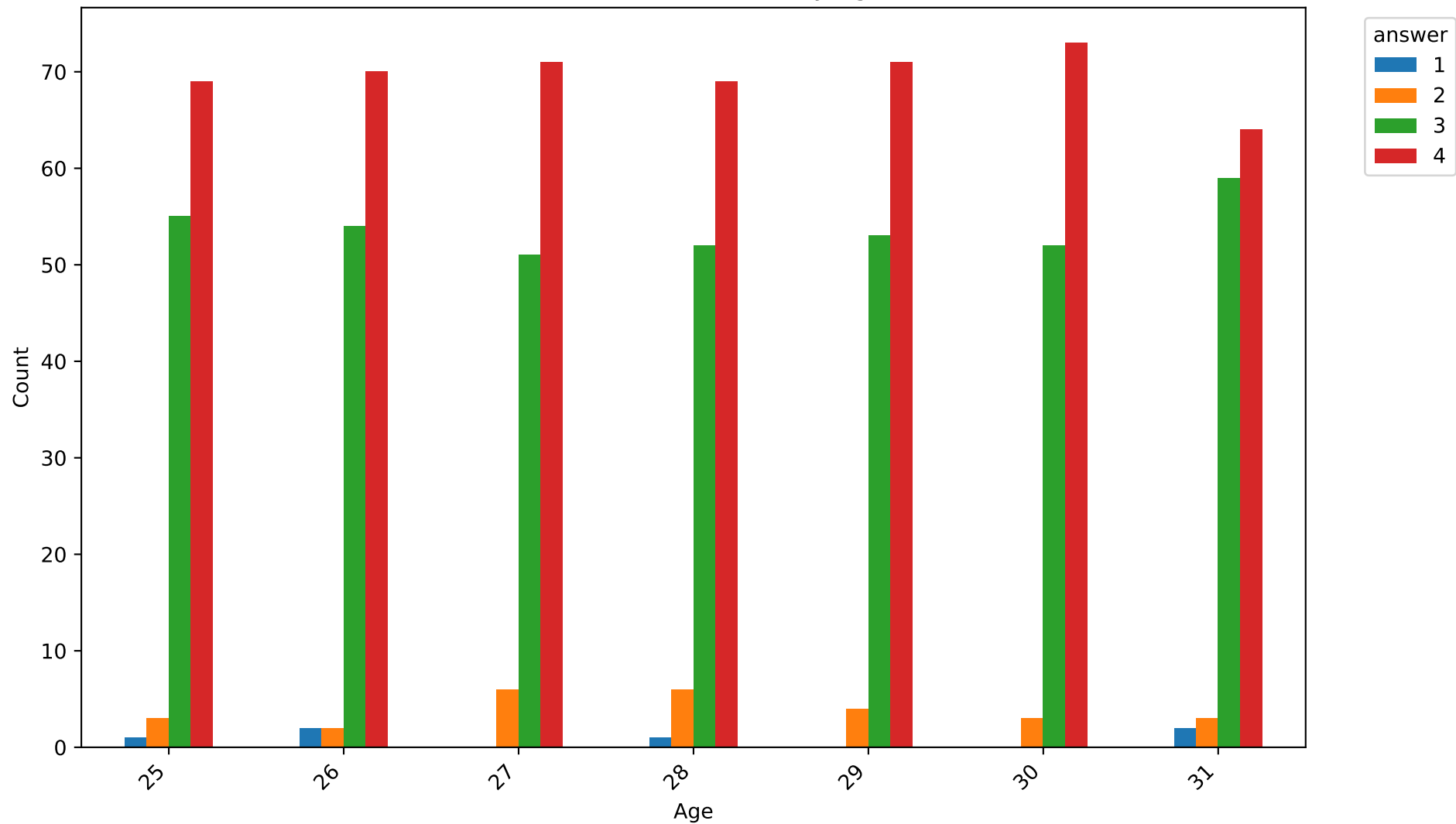
Distribution of 'answer' by Age
