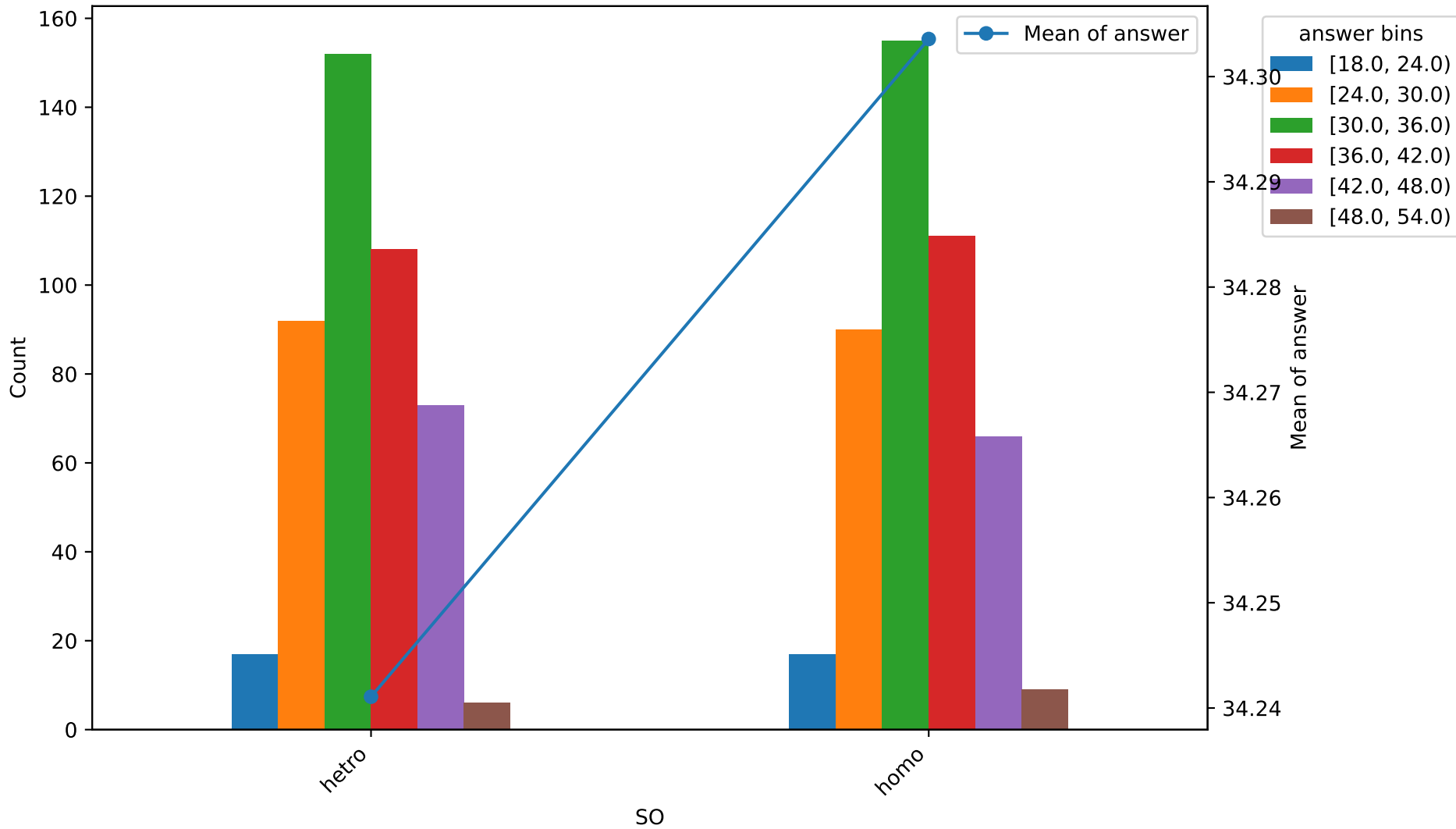
Binned distribution of 'answer' (bin=6.0) and mean by SO
