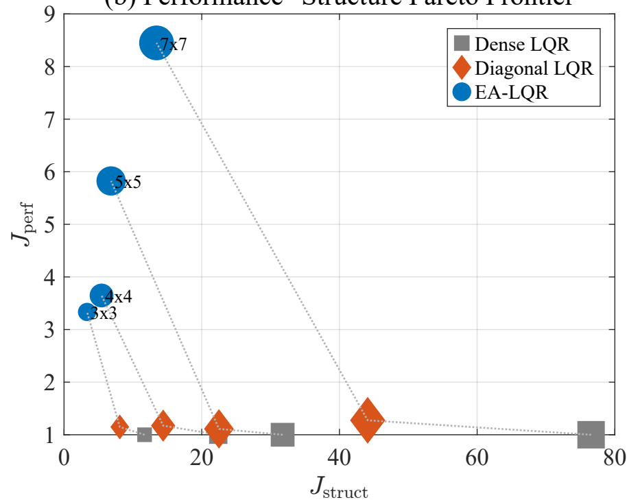
(b) Performance--Structure Pareto Frontier
