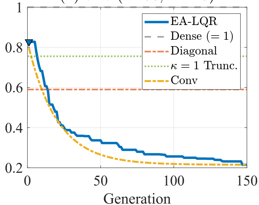
(e) 7 \times 7 EA controller
