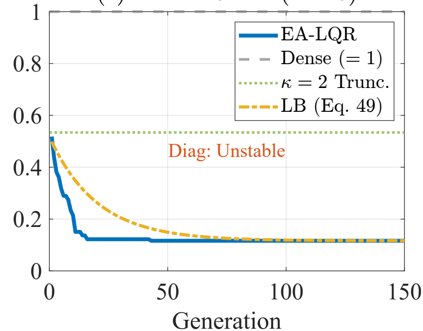
(f) IEEE 13-bus EA controller
