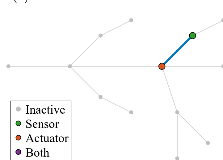
(f) IEEE 13-bus EA controller
