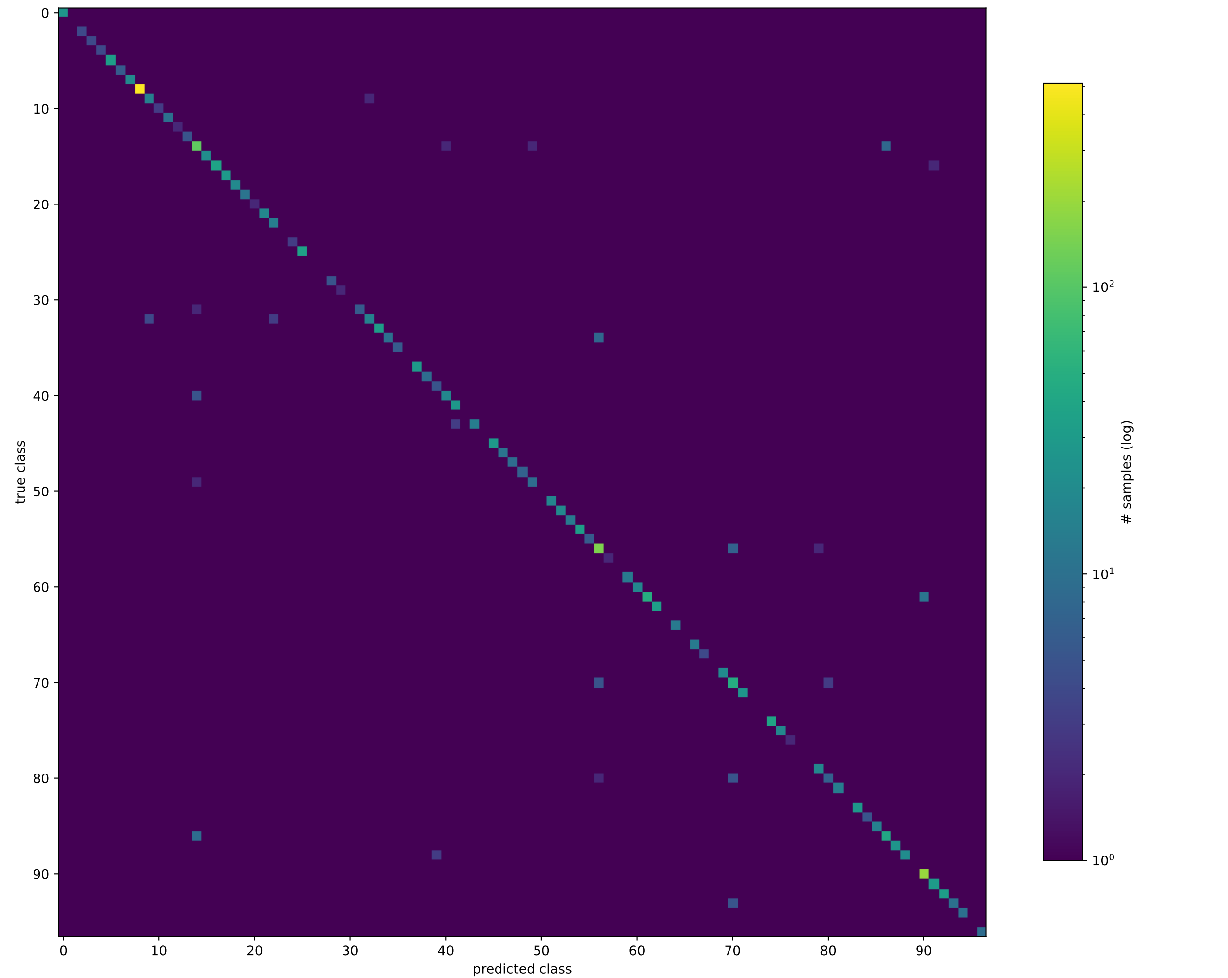
acc=94.79 bal=91.48 macF1=92.25
