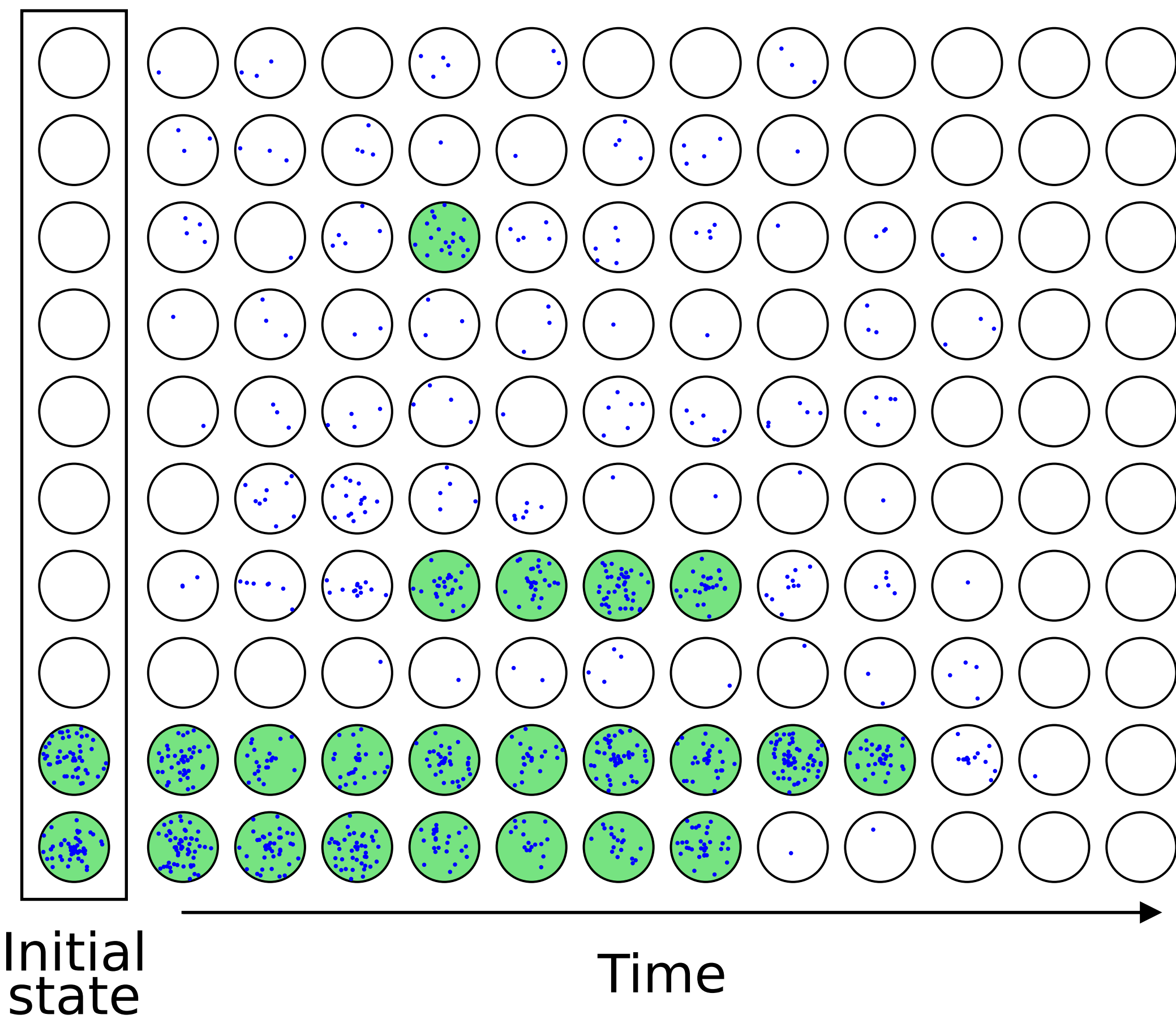
(b) Insufficient initial regional abundance
