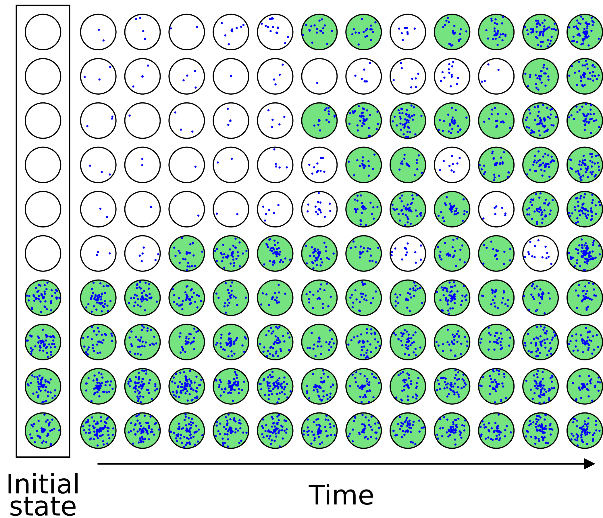
(a) Sufficient initial regional abundance
