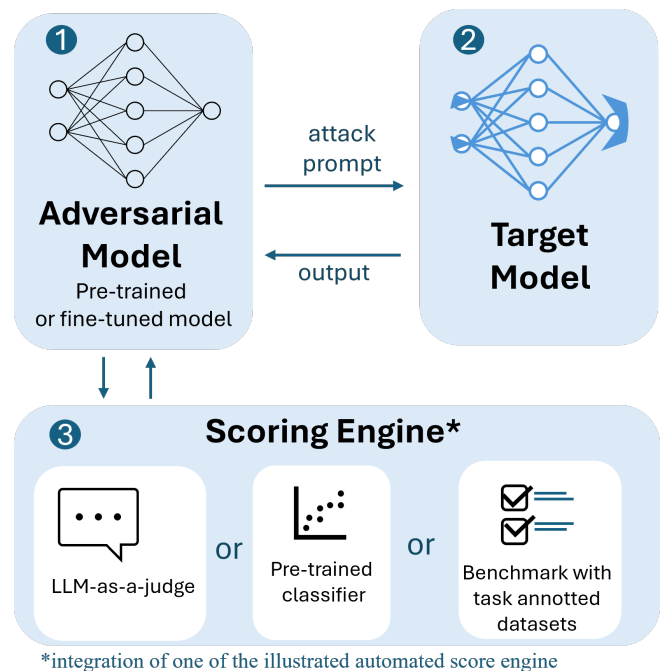
FIGURE 8. Key Elements of Recent Automated Red Teaming Architectures for LLMs
