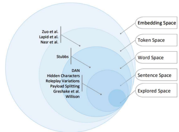
FIGURE 4. Visualization of the Prompt Injection Space as proposed by Kumar et al. 2024 a , illustrating five levels of abstraction: embedding, token, word, sentence, and explored spaces.
