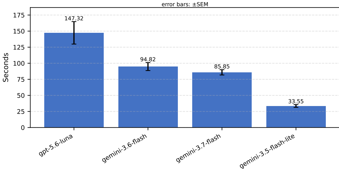
models: Elapsed time (totaller+reflective-loop, grouped by model)
