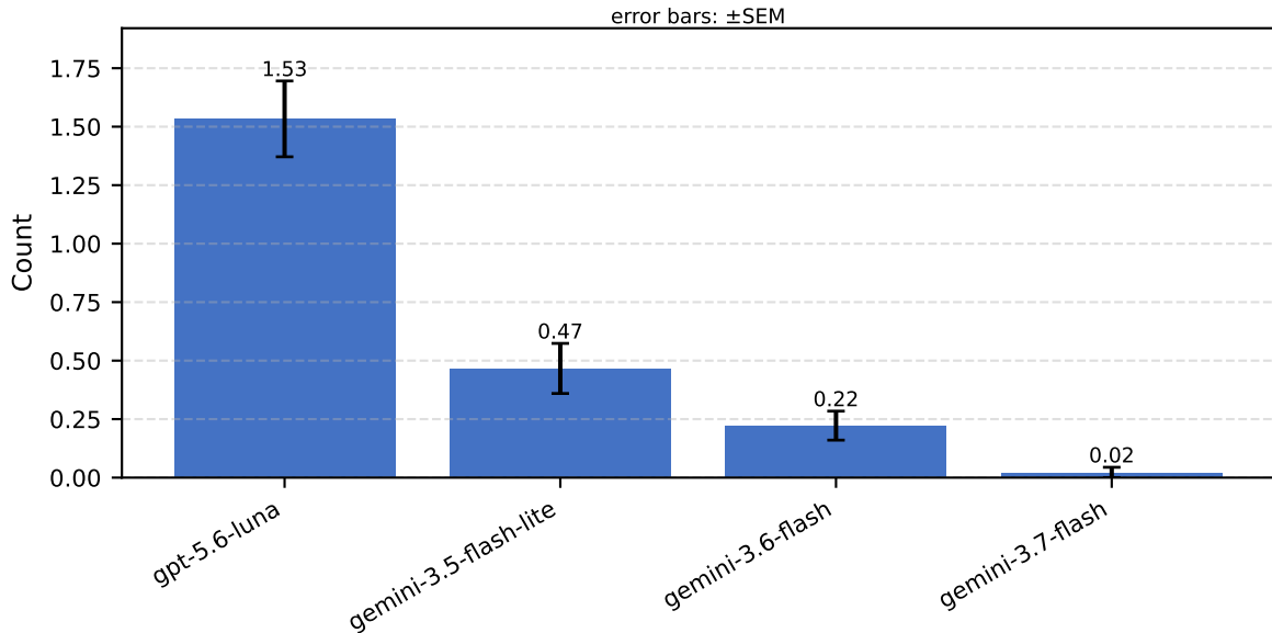
models: Iterations (totaller+reflective-loop, grouped by model)
