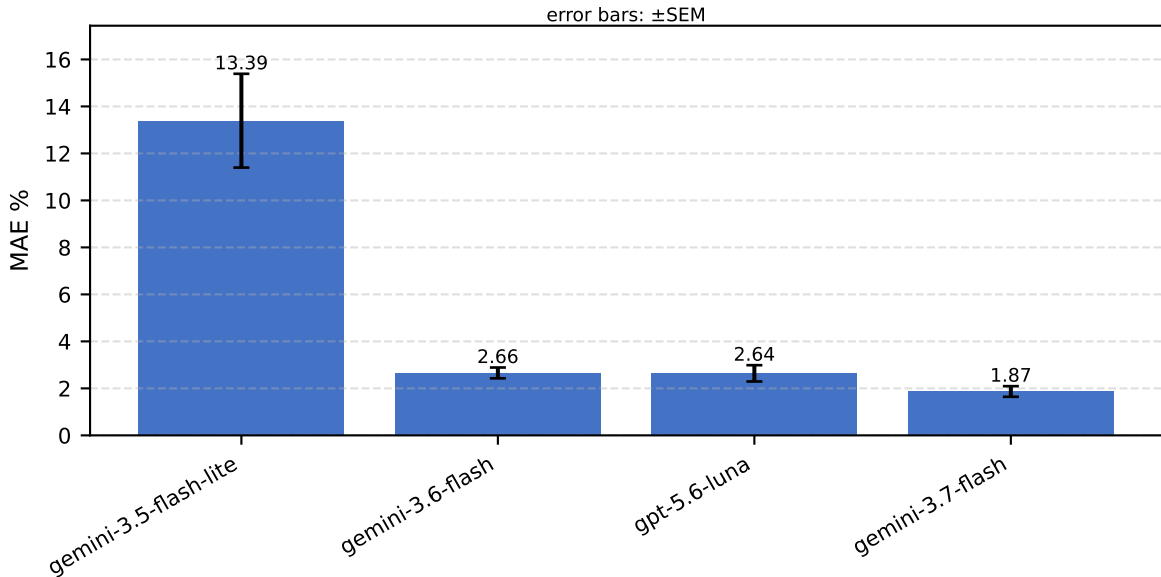
models: Macro MAE % (totaller+reflective-loop, grouped by model)
