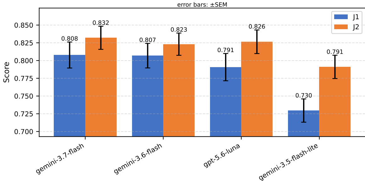
models: Soft preference aggregate (totaller+reflective-loop, grouped by model)
