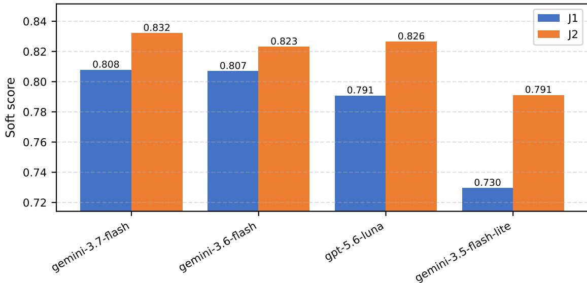
Experiment 2: Soft score (grouped by model)
