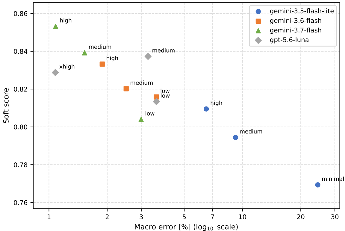
Experiment 2: Macro error vs soft score (J2)
