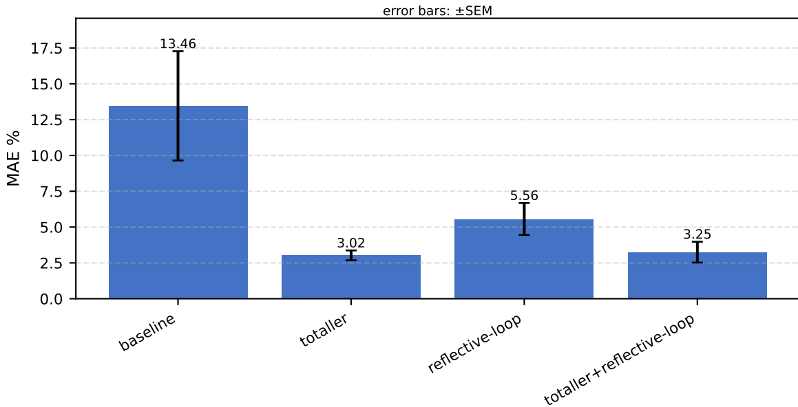
ablation: Energy and macronutrient MAE % (gpt-5.6-luna)
