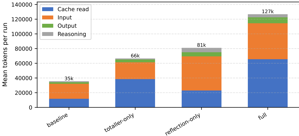
Experiment 1: Token spend
