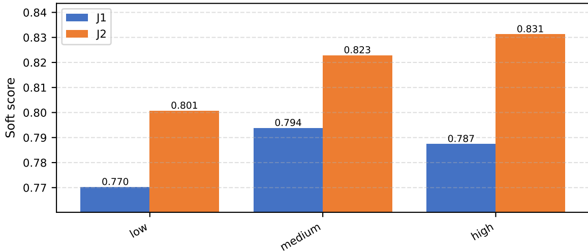
Experiment 2: Soft score (grouped by effort)
