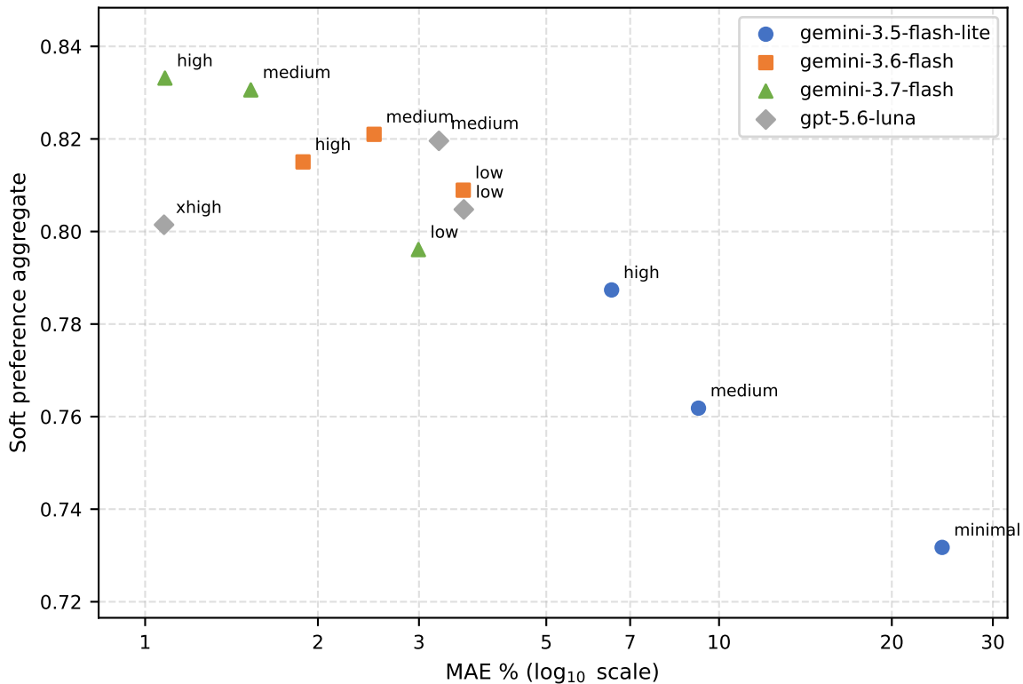
models: MAE vs soft preference (mean of J1 and J2)
