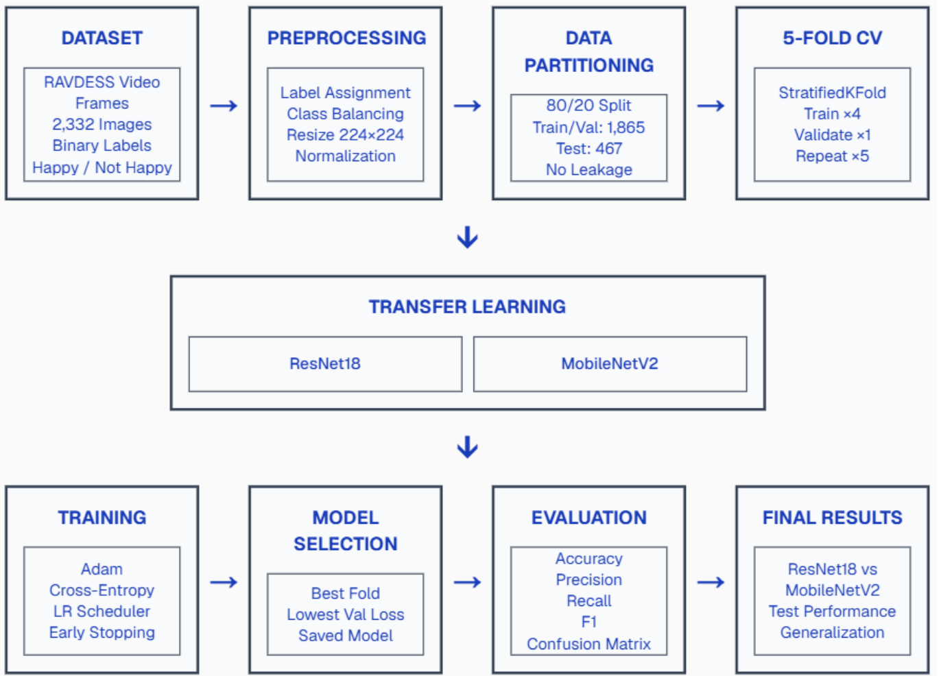
Fig. 1. Overall workflow of the proposed transfer learning framework, including data preprocessing, dataset partitioning, transfer learning with ResNet18 and MobileNetV2, stratified 5-fold cross-validation, and final model evaluation.
