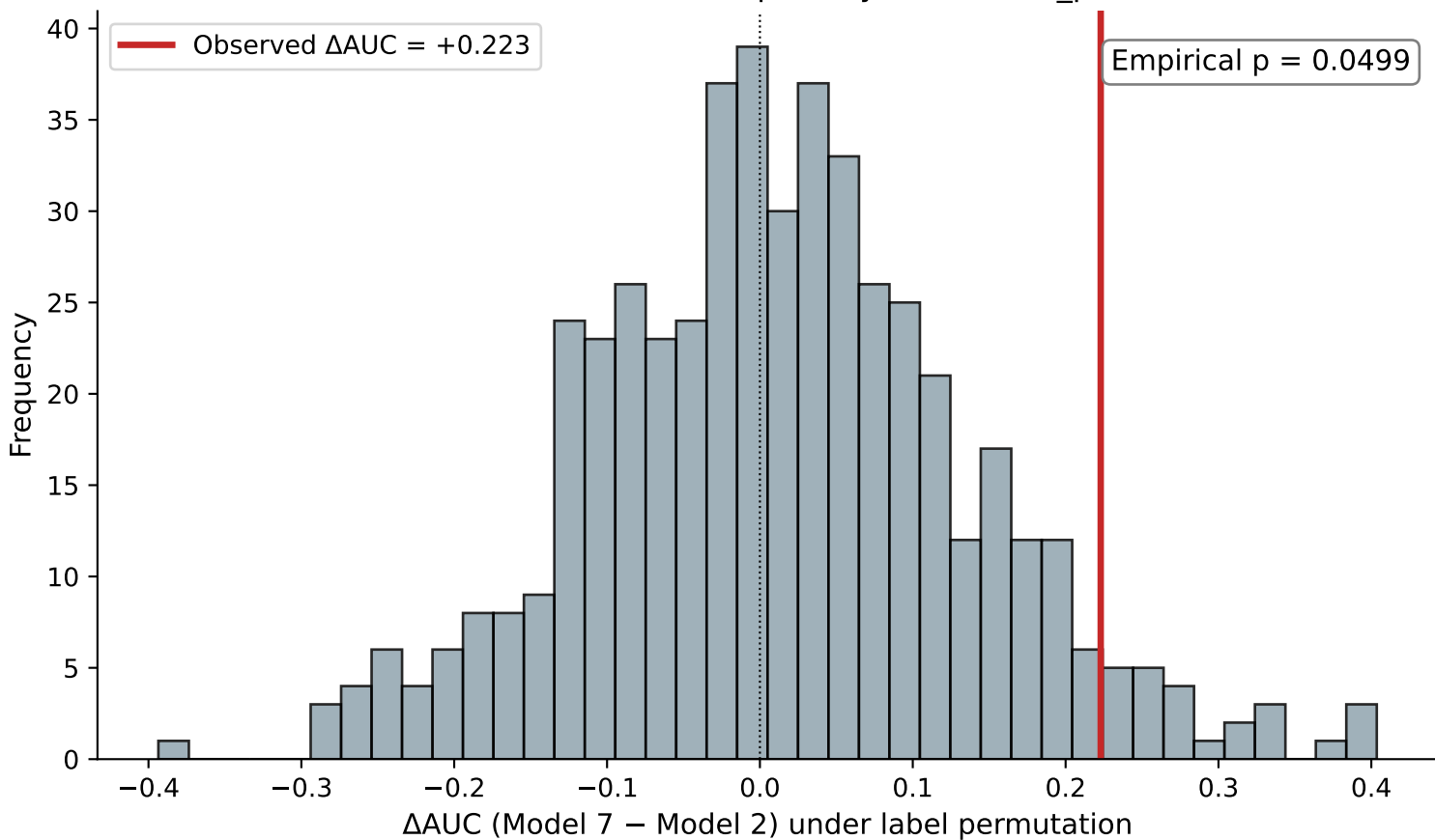
Permutation null distribution — primary contrast ( n_{\text{perm}} = 500 )
