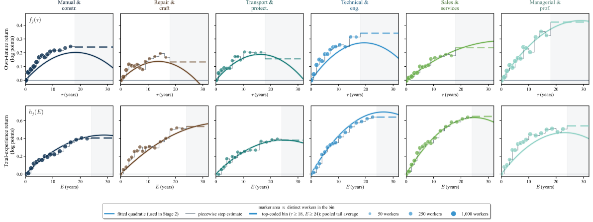
Figure 9: Stepwise versus quadratic returns to tenure for each cluster. The quadratic specification attains a log-likelihood of -38,167.82 against -38,045.19 for the stepwise specification, but the stepwise specification has 162 additional parameters.
