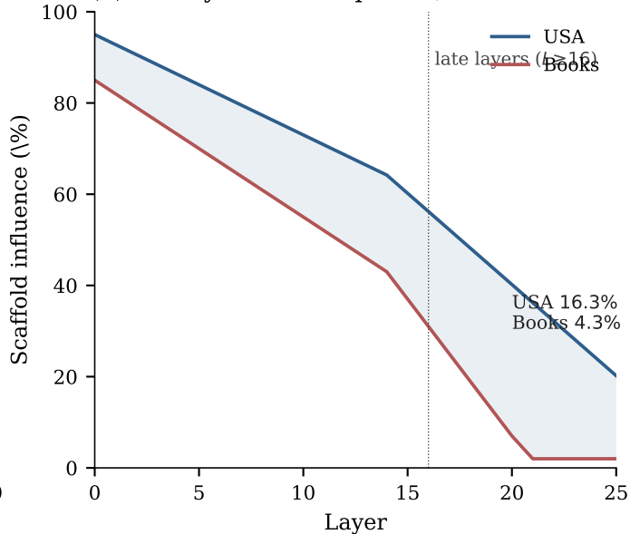
(b) Per-layer scaffold profile, USA vs Books
