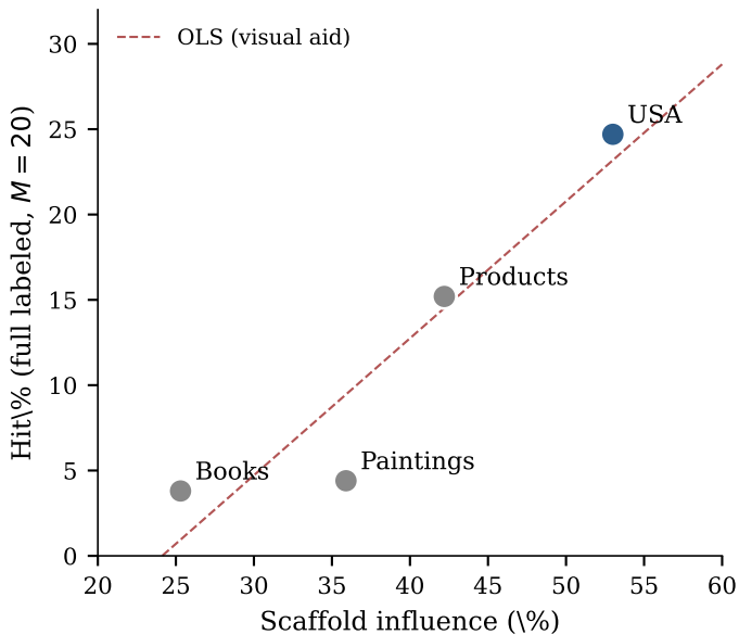
(a) Cross-domain scaffold \rightarrow Hit\% ( \rho = 1.0 , N = 4 )
