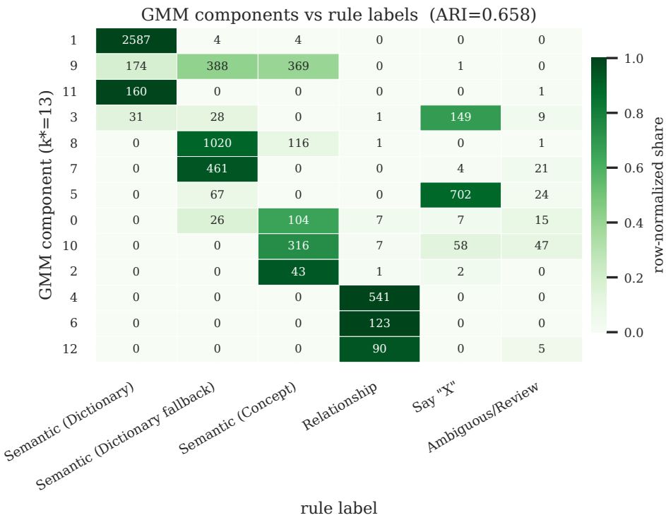
BIC-preferred Gaussian mixture
