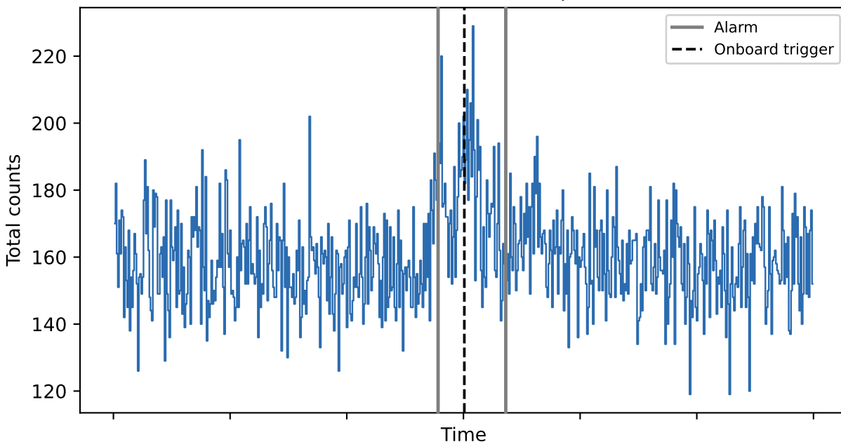
NPFOCuS on GRB total counts (Poisson-sampler calib.)
