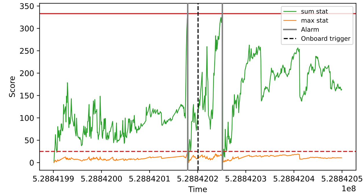
NPFOCuS statistics and thresholds
