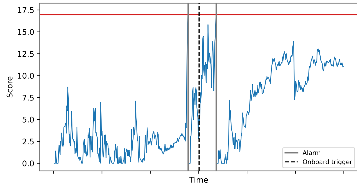
NPFOCuS statistics and thresholds
