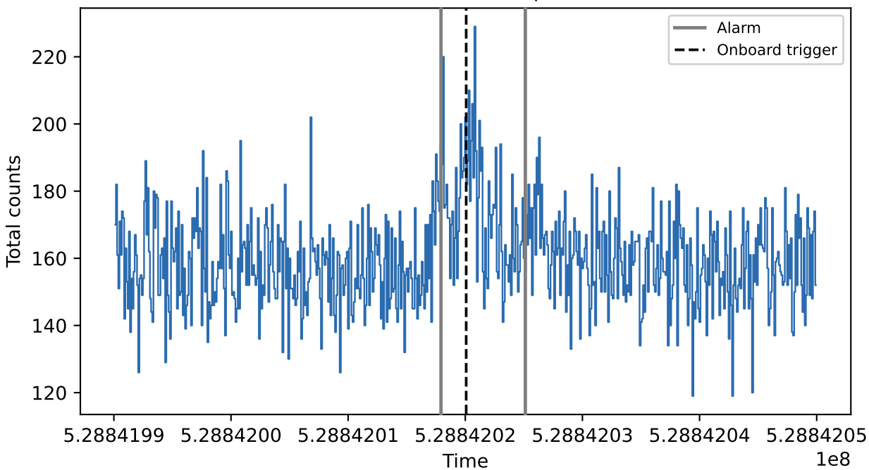
NPFOCuS on GRB total counts (Poisson-sampler calib.)
