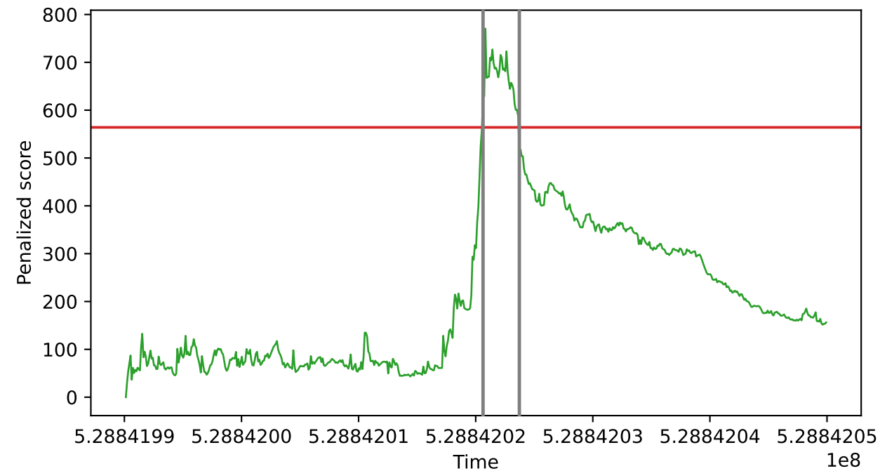
NPFOCuS sum statistic and threshold
