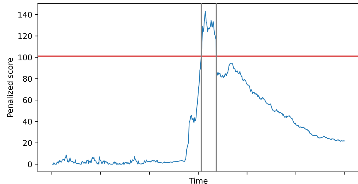
NPFOCuS sum statistic and threshold
