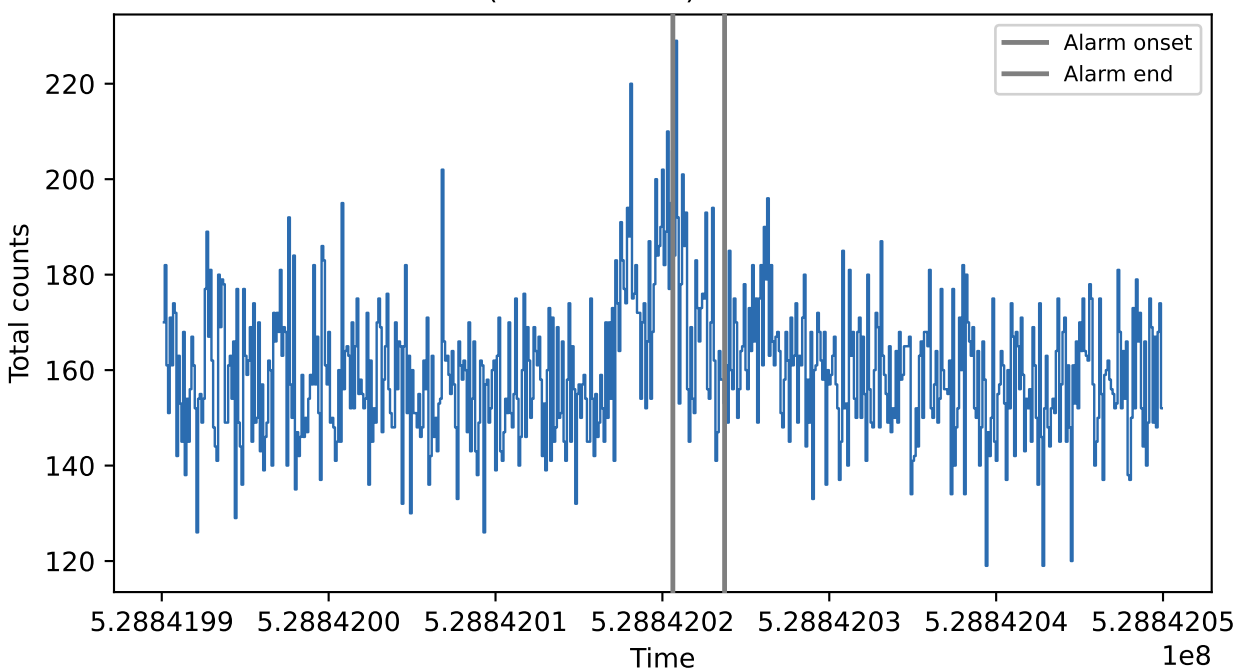
NPFOCuS on GRB counts (sum statistic)
