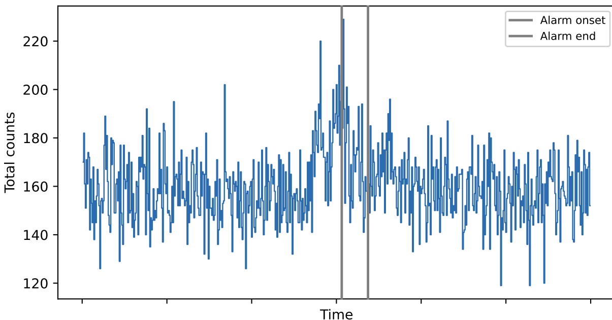
NPFOCuS on GRB counts (sum statistic)
