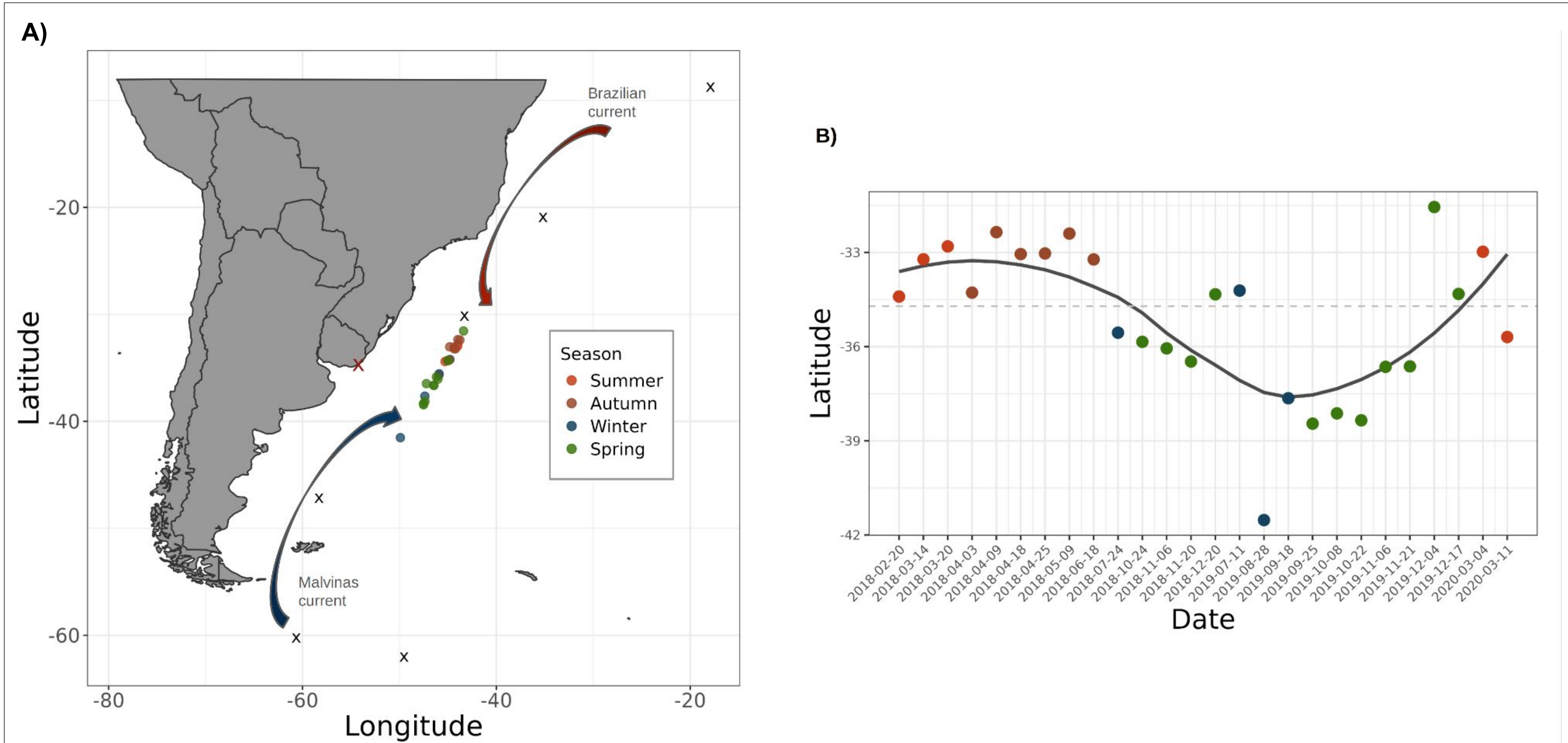
Figure 2. Community differentiation linked to ocean current dynamics. A) Space-time analysis of SAMO. SAMO samples were positioned relative to six South Atlantic TARA sites (1) using Bray-Curtis similarity of genus profiles. SAMO coordinates were calculated as weighted averages of TARA locations, weighted by Bray-Curtis similarity. Black crosses mark TARA sites, the red cross marks SAMO, colours indicate seasons. Brazil and Malvinas currents are shown schematically. B) Scatterplot showing variability of the imputed latitude coordinate over time, with a LOESS regression line.
