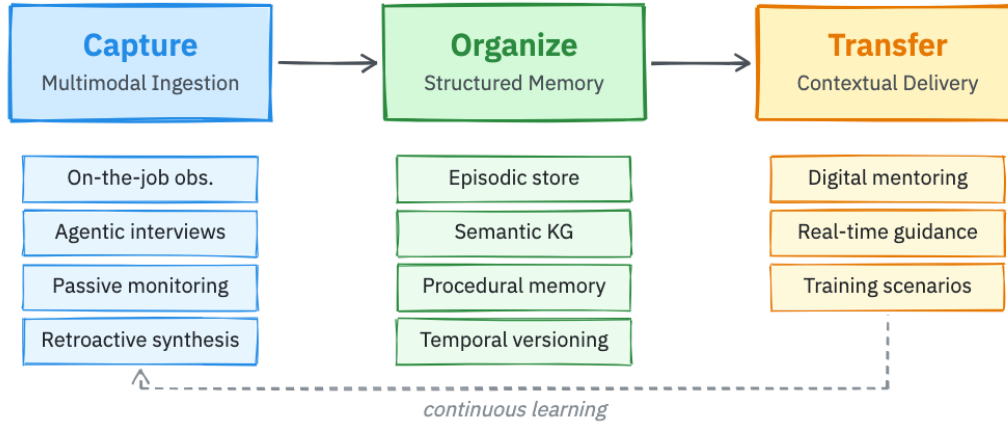
Figure 1: The CAPTURE–ORGANIZE–TRANSFER framework. A feedback loop enables the agent to refine its knowledge continuously from new worker interactions.
