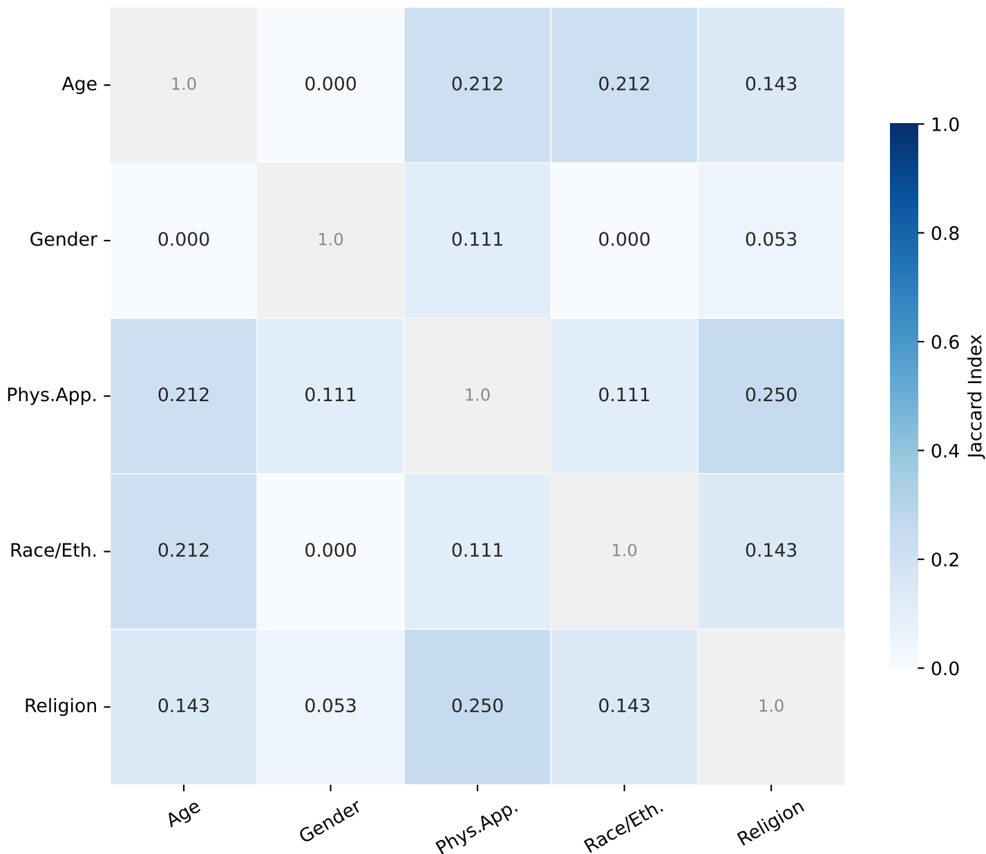
Jaccard Overlap — Llama-3.2-1B | English | Top-20 neurons (abs.)
