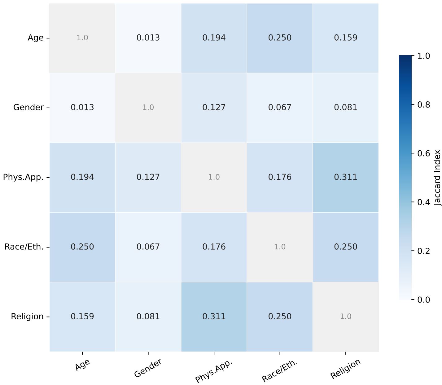
Jaccard Overlap — Llama-3.2-1B | English | Top-40 neurons (abs.)
