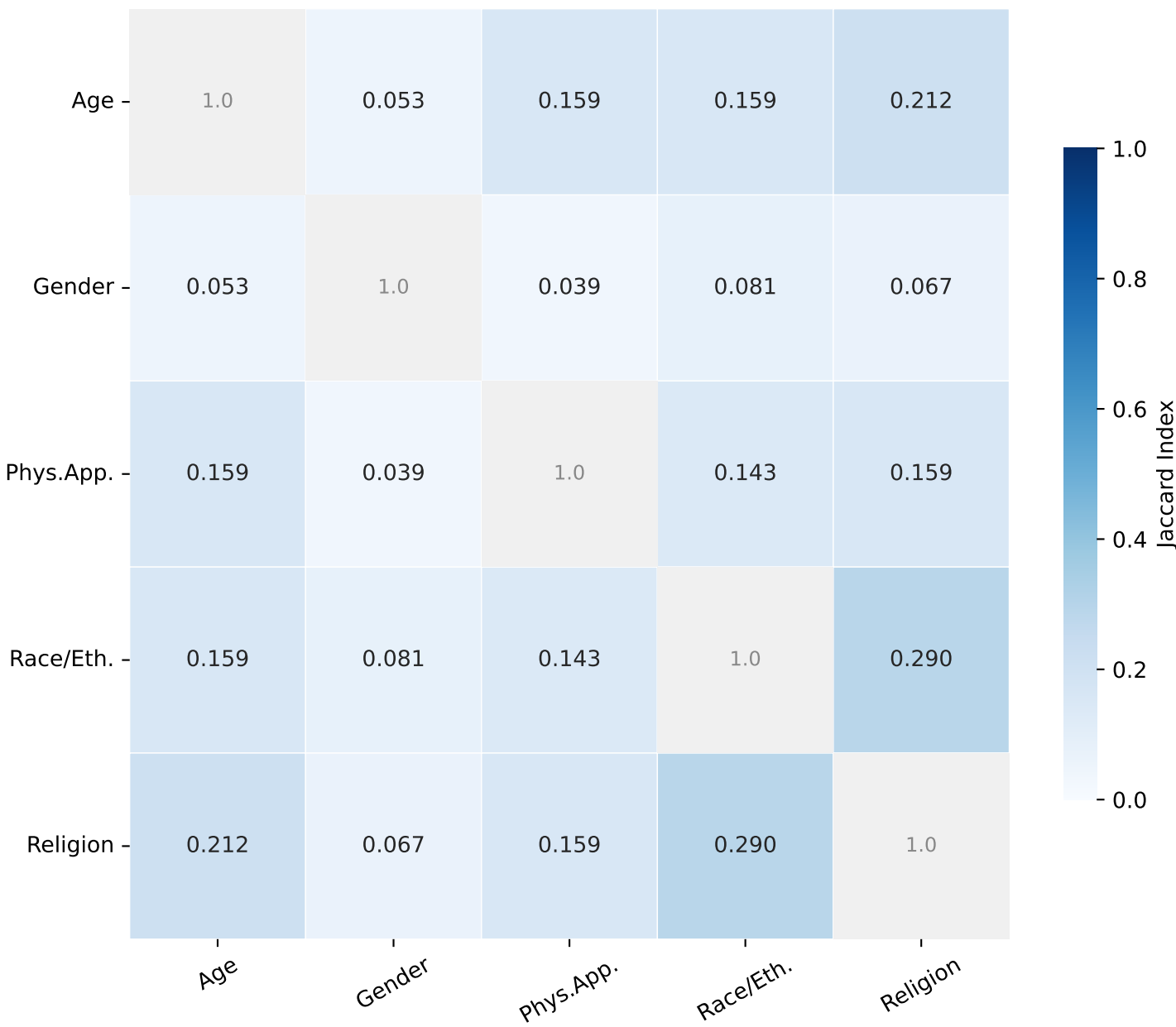
Jaccard Overlap — Llama-3.2-1B | Spanish | Top-40 neurons (abs.)
