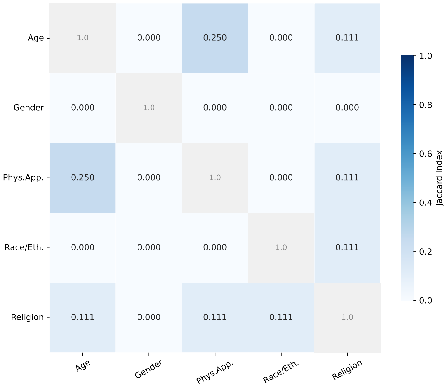
Jaccard Overlap — Llama-3.2-1B | Spanish | Top-5 neurons (abs.)
