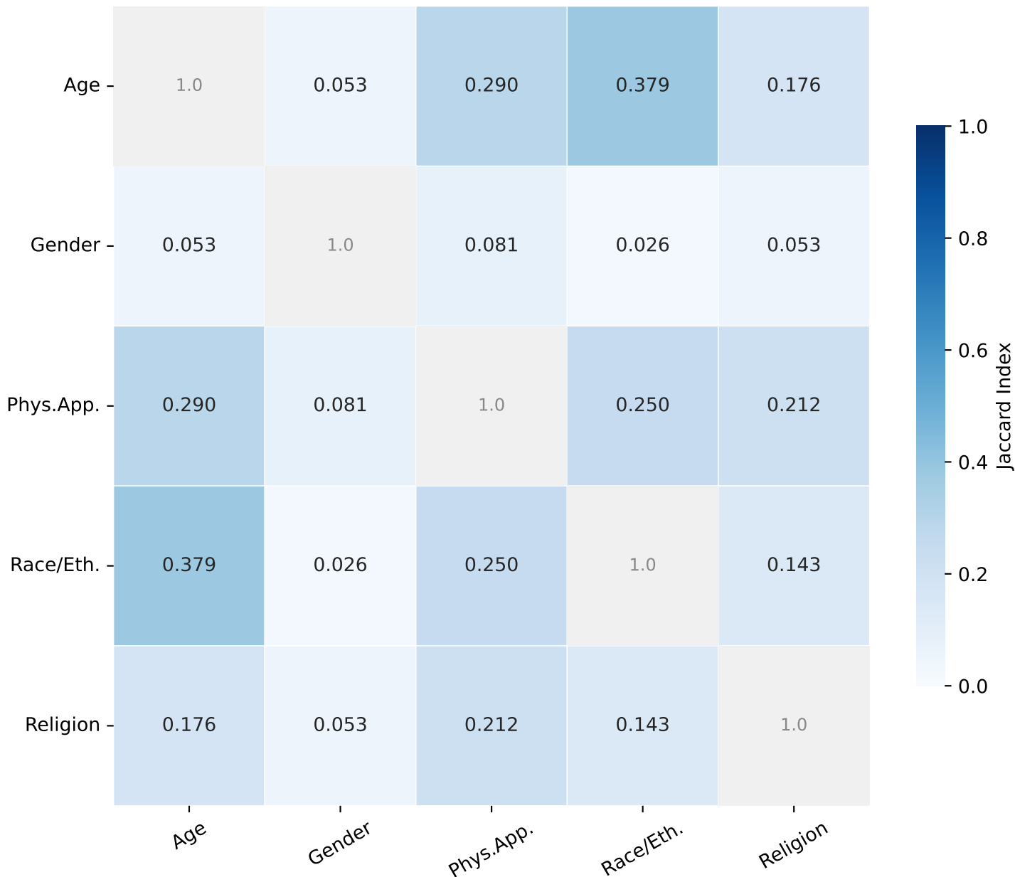
Jaccard Overlap — Llama-3.2-3B | English | Top-20 neurons (abs.)
