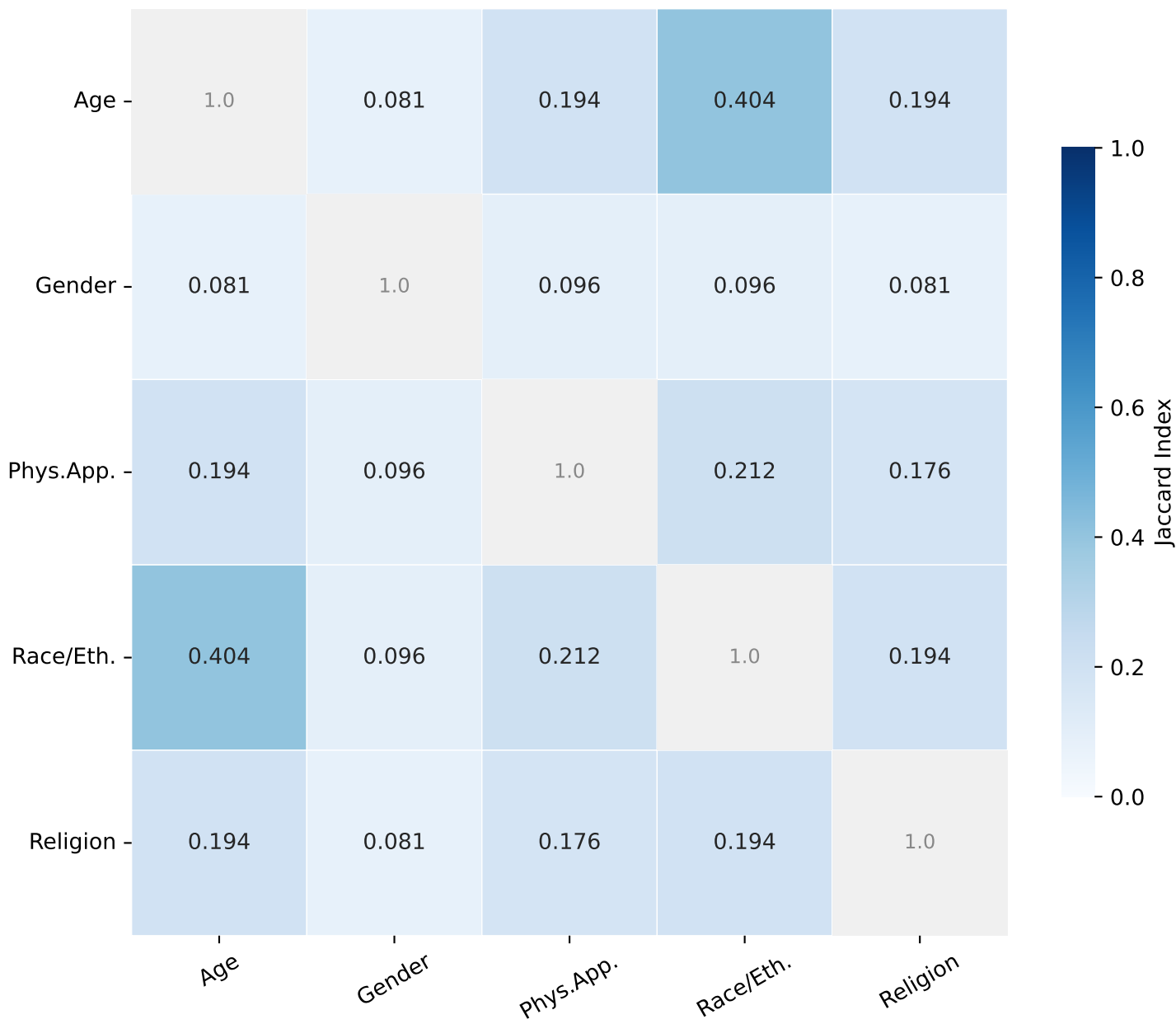
Jaccard Overlap — Llama-3.2-3B | English | Top-40 neurons (abs.)
