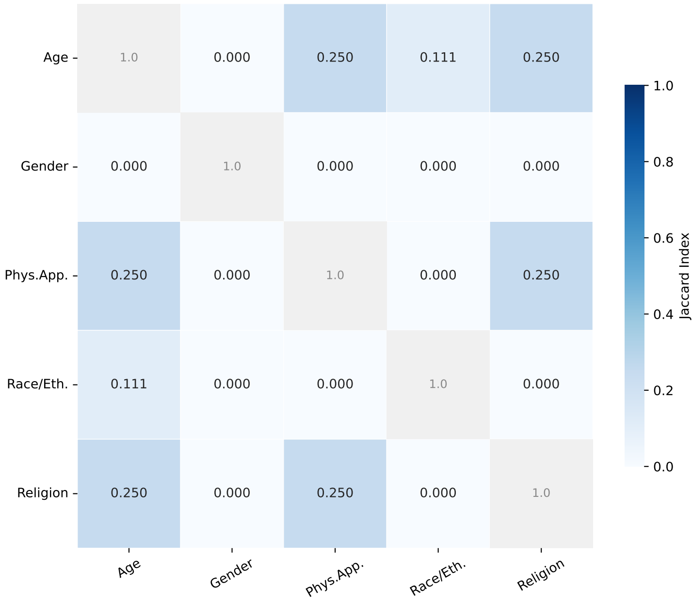
Jaccard Overlap — Llama-3.2-3B | English | Top-5 neurons (abs.)
