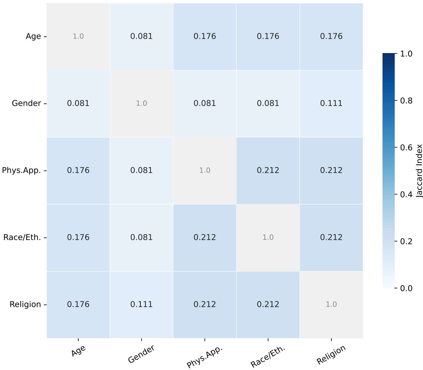
Jaccard Overlap — Llama-3.2-3B | Spanish | Top-40 neurons (abs.)
