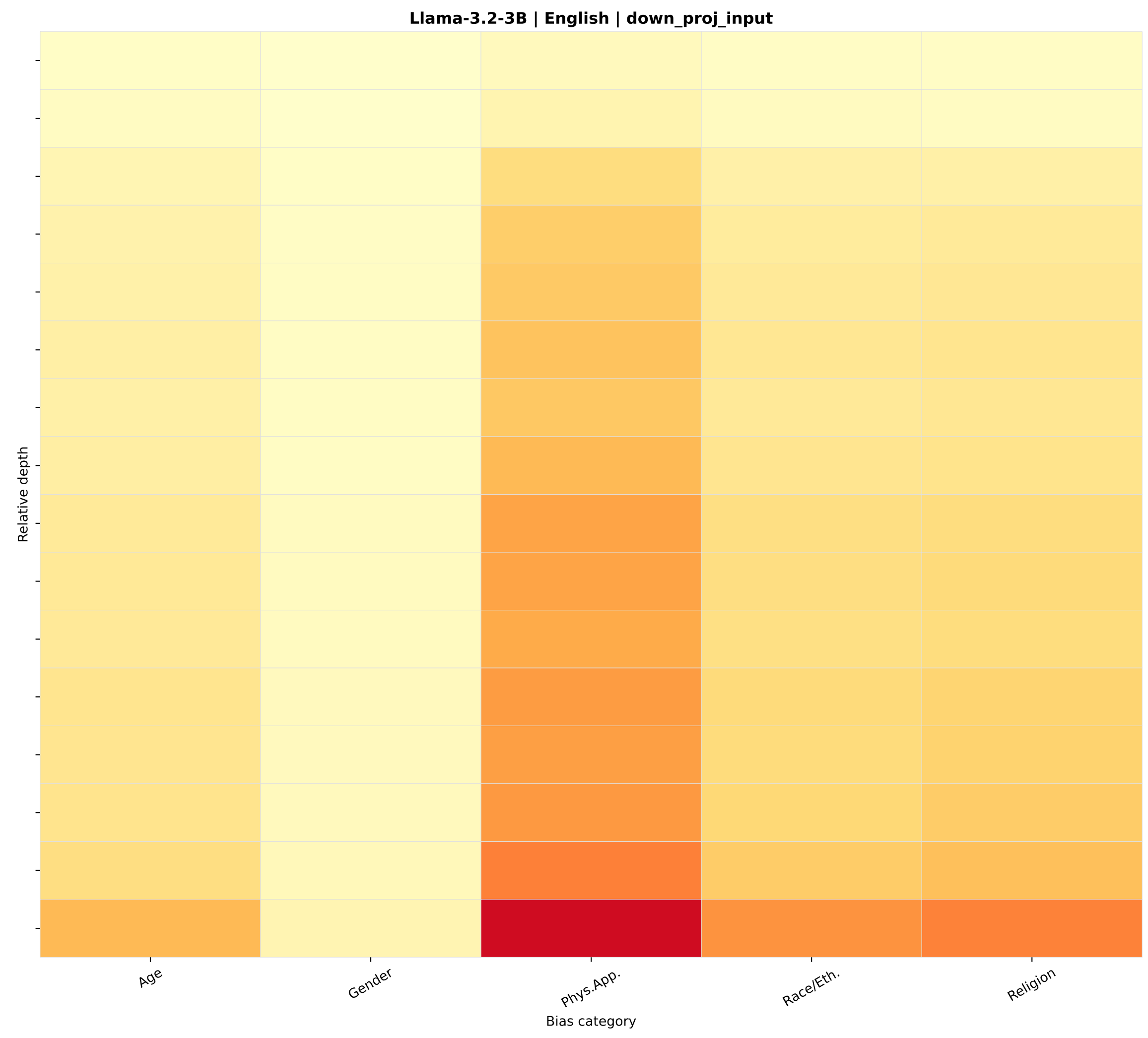
Bias Path Comparison — English | down_proj_input
