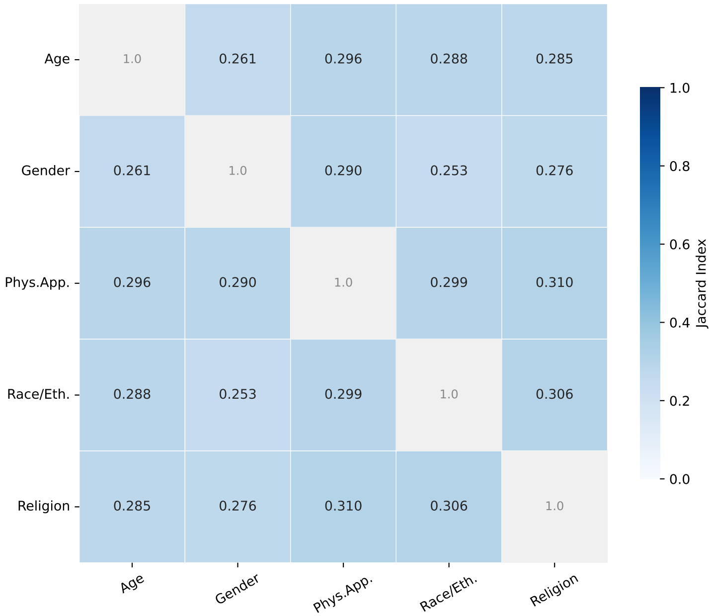
Jaccard Overlap — Llama-3.2-1B | English | Top-5%
