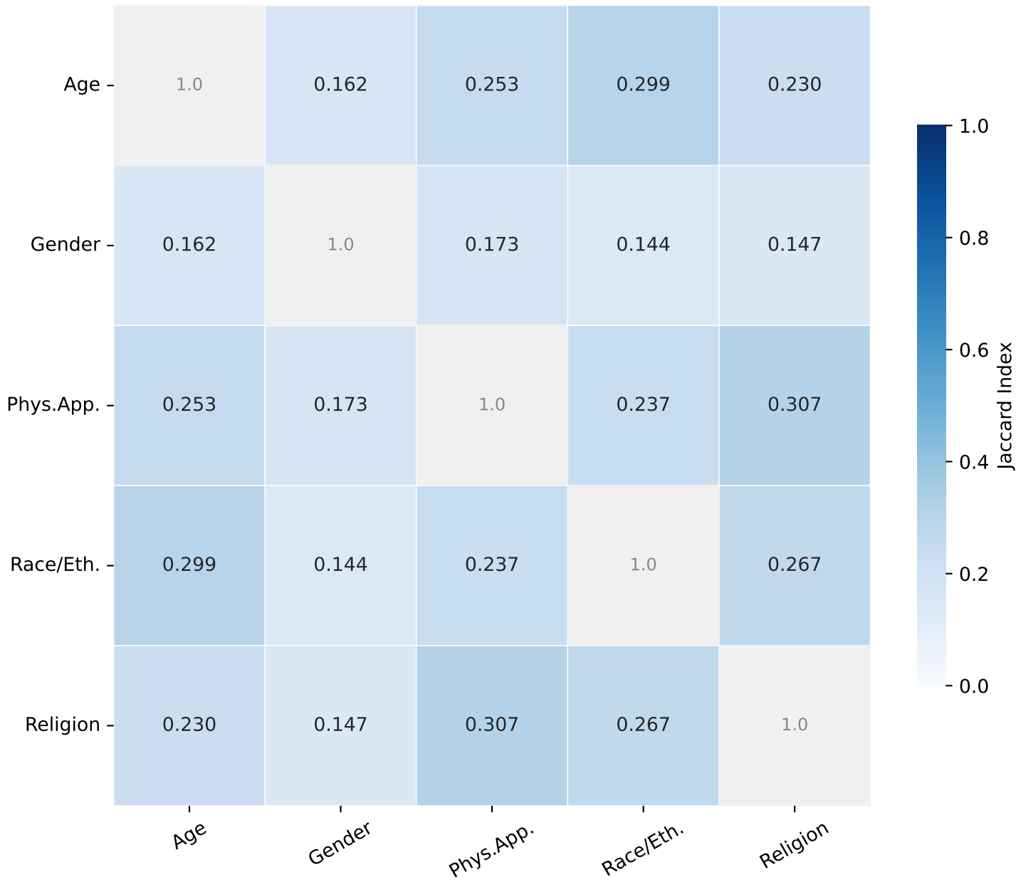
Jaccard Overlap — Llama-3.2-3B | English | Top-0.1%
