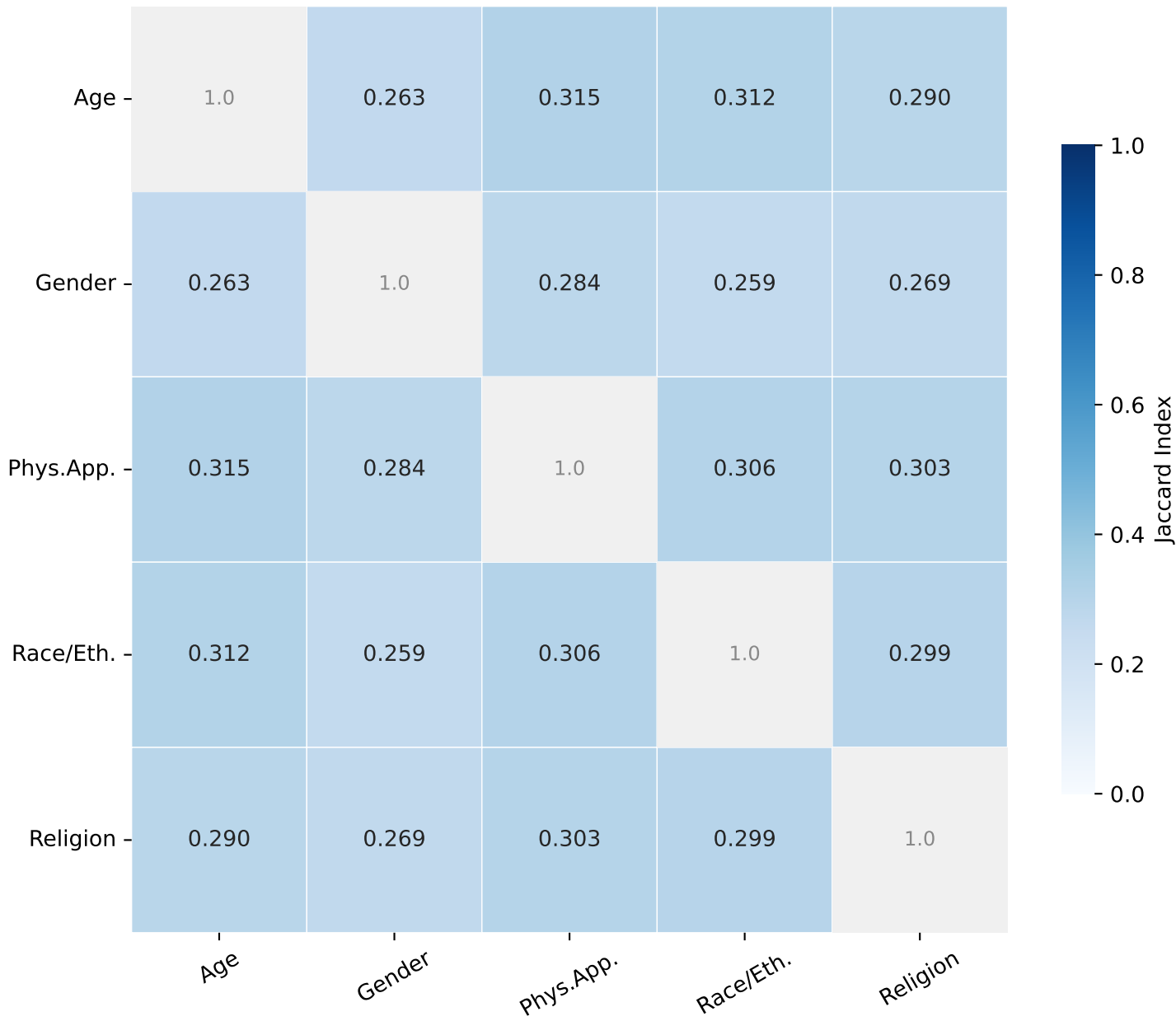
Jaccard Overlap — Llama-3.2-3B | English | Top-5%
