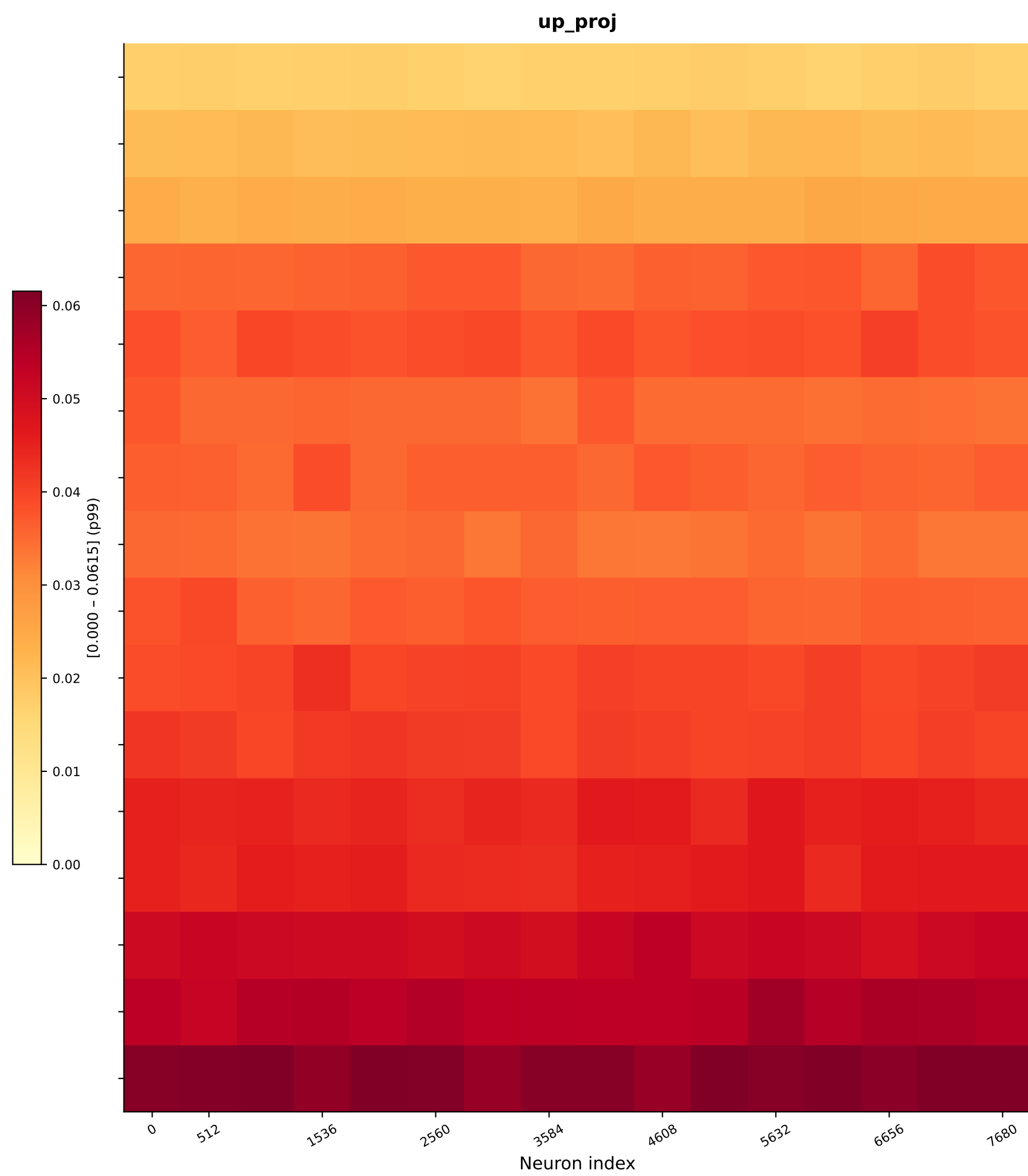
Neuron Bias Heatmap — Llama-3.2-1B | English | Age | bin=512
