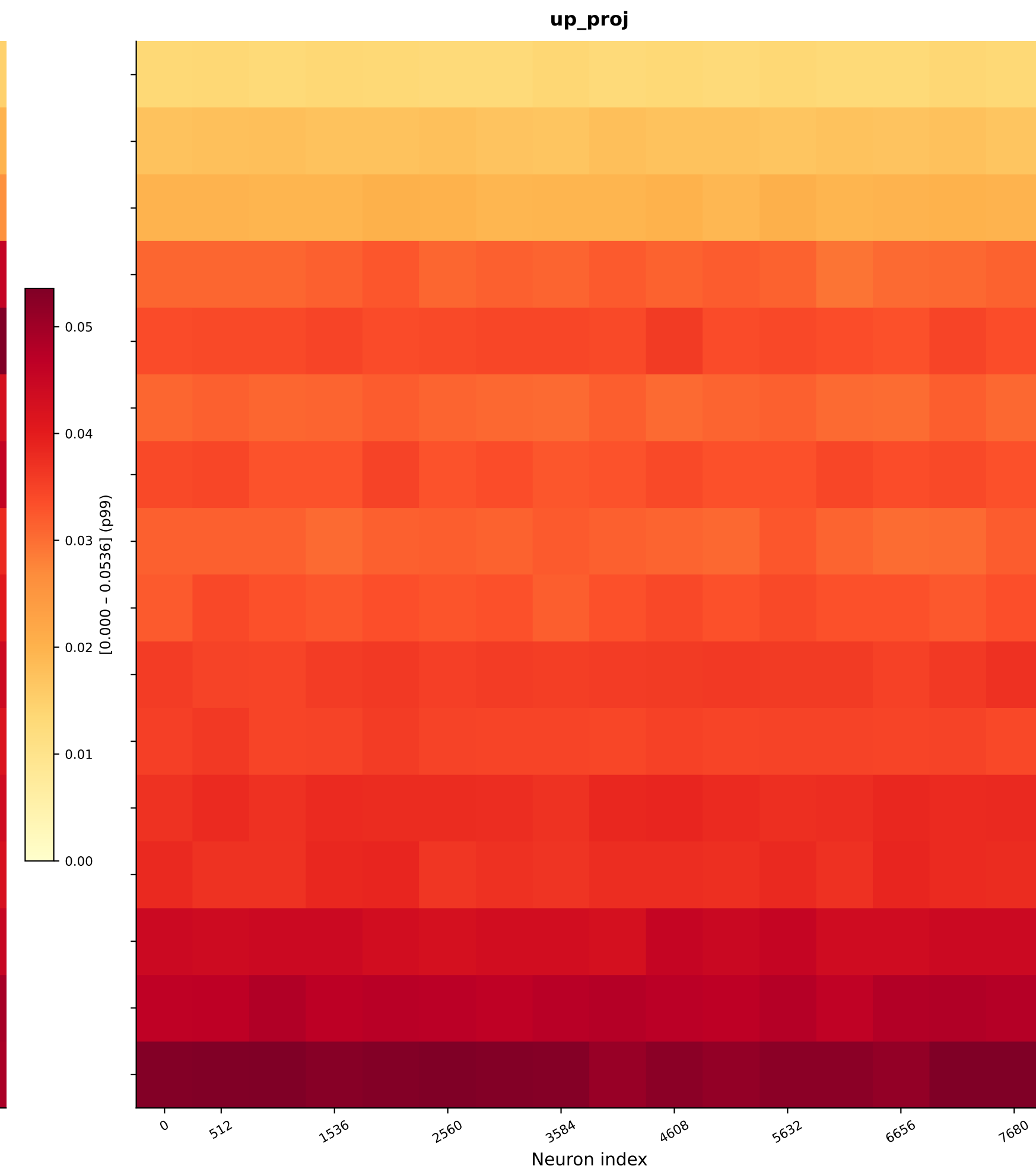
Neuron Bias Heatmap — Llama-3.2-1B | English | PhysicalAppearance | bin=512
