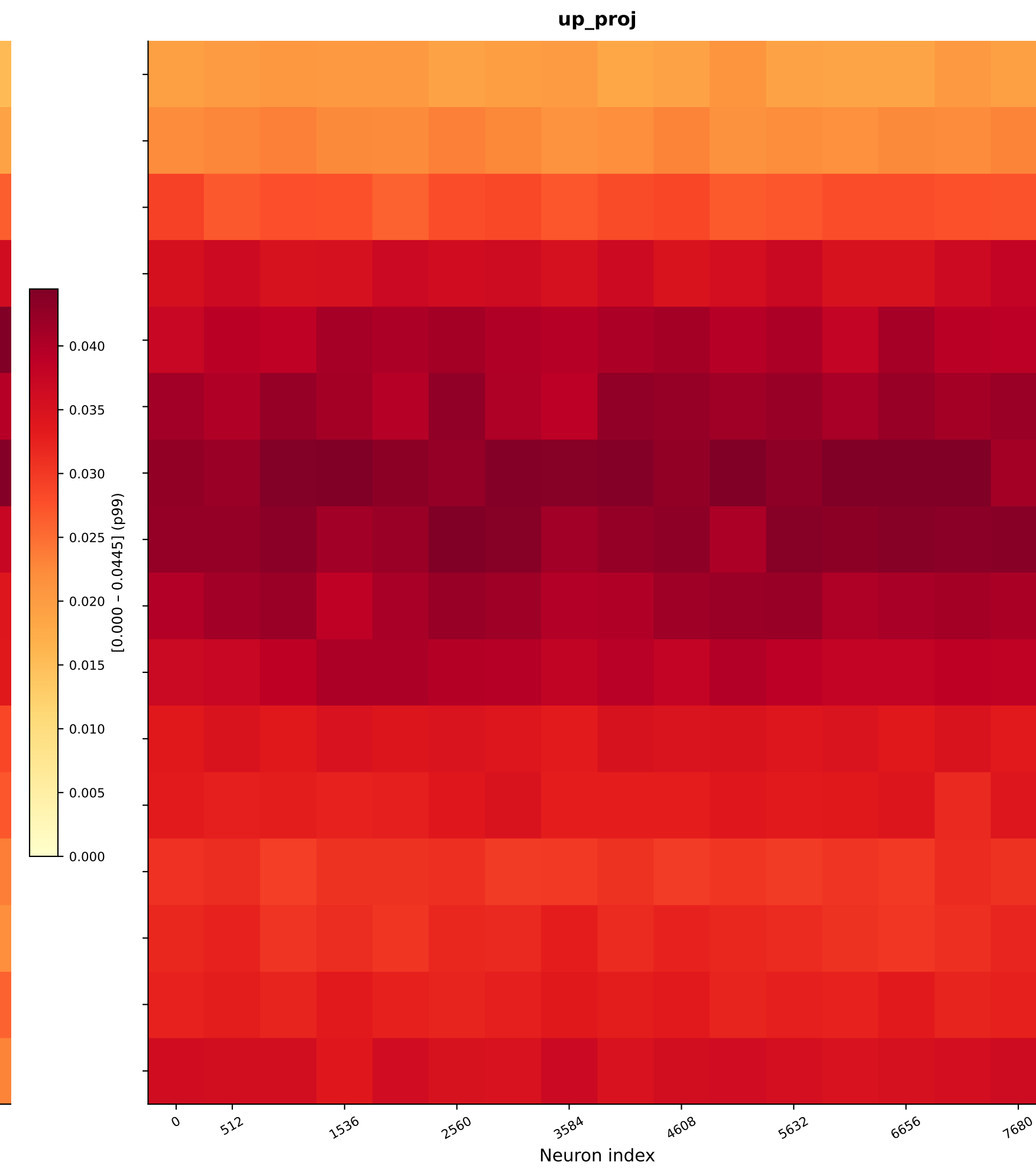
Neuron Bias Heatmap — Llama-3.2-1B | Spanish | Age | bin=512
