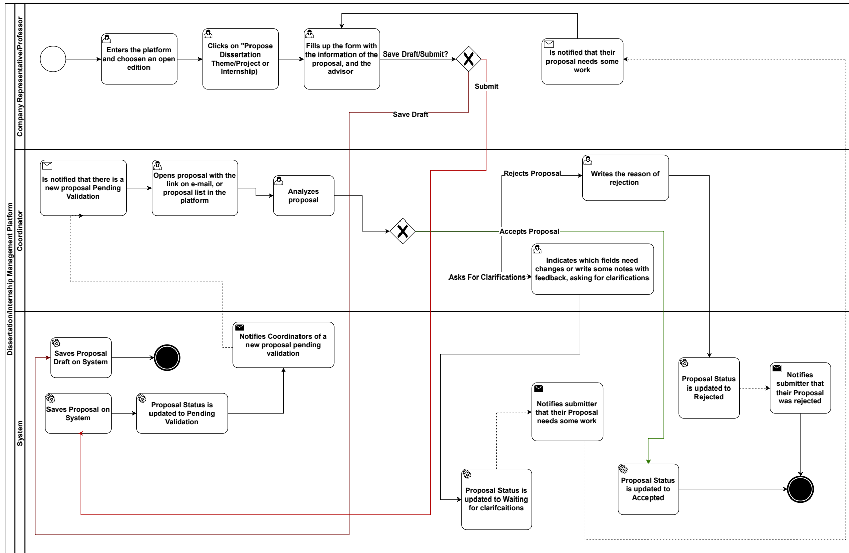
Figure C.2: BPMN diagram of the proposal submission and validation workflow between company /professor, coordinator, and the platform
